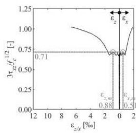
Homogeneous in-plane shear with imposed longitudinal strain (Beck 2020)
