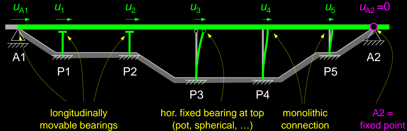
Movements due to girder contraction (schematic, horizontal fixity at right abutment A2)
