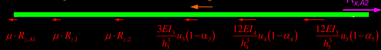
Loads on girder
