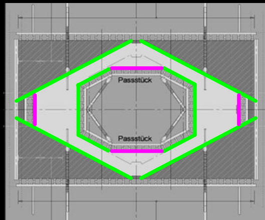
formwork panels used for full pier height
