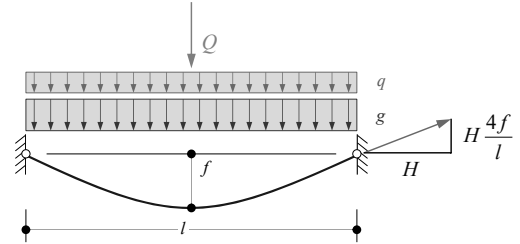
Estimation of suspension cable force (parabolic sag)
