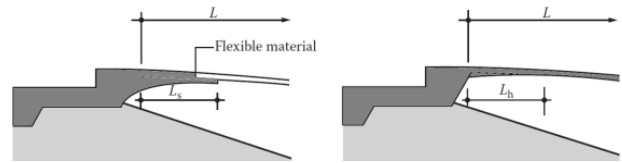
End support details for stress-ribbon bridges [Strasky 2004]
