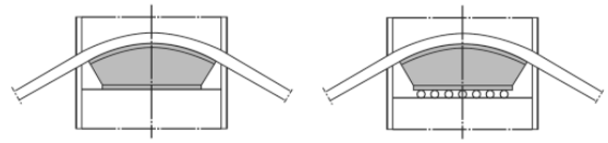
Tower saddle of Third Bosphorus Bridge
