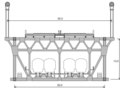
Bisan-Seto suspension bridges (1988, spans 990/1100 m)
