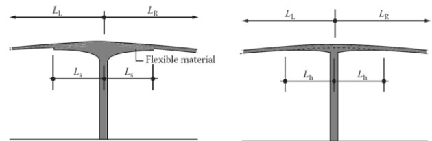
Pier support details for stress-ribbon bridges [Strasky 2004]
