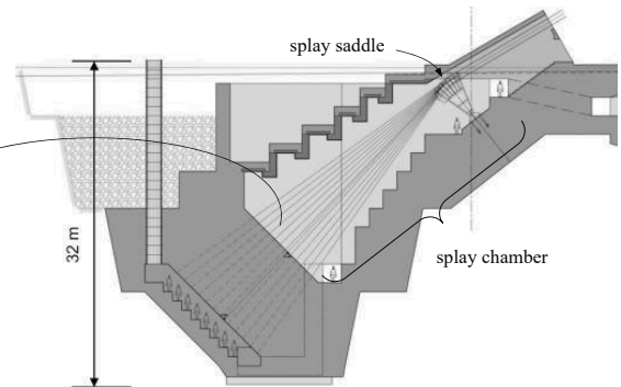
Splay chamber of 3 rd Bosphorus Bridge [Klein+Delémont, 2016]
