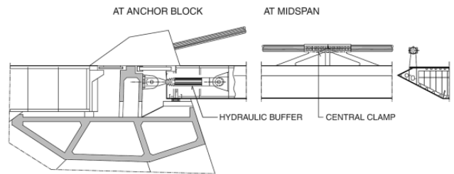
Example of hydraulic buffers at anchor blocks and central clamp (Storebaelt bridge [Gimsing 2012])
