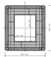
Tower of Storebælt bridge (1998) [Gimsing 2012]
