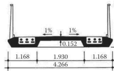
Typical cross-section [Strasky 2004]
