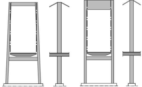
Tower geometries for continuous stiffening girder [Gimsing 2012]
