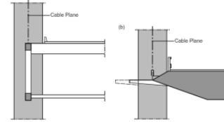
Tower geometries for continuous stiffening girder [Gimsing 2012]
