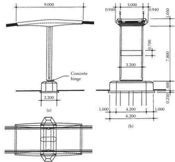
Pier of Prague-Troja stress-ribbon bridge [Strasky 2004]
