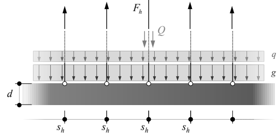
Estimation of hanger forces [Gimsing 2012]
