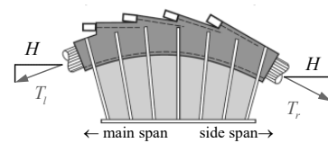
Saddle with additional strands for side span cable, anchored on the saddle above continuous strands [Gimsing 2012]
