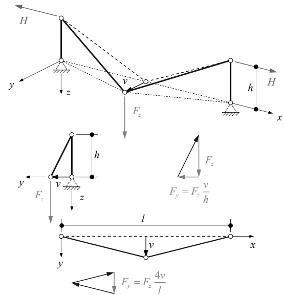
Contribution of cable system to transfer of transverse loads
