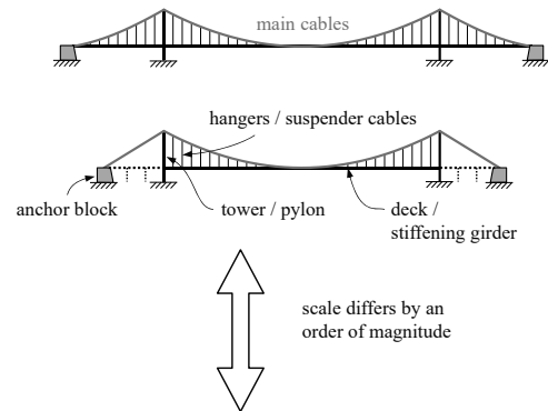
Suspended bridge / Stress-ribbon (Spannband)
