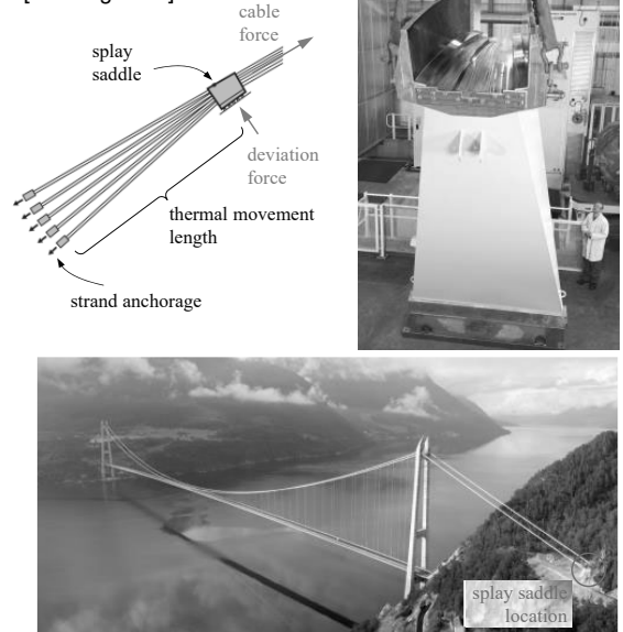
Splay saddle: Elevation and example (Hardanger bridge) [Gimsing 2012]
