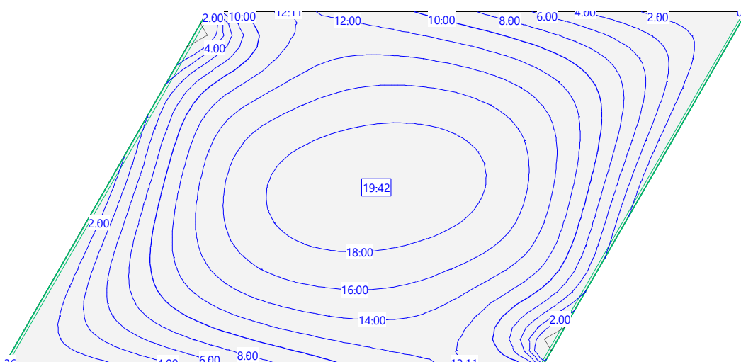
Figure 11: Cross-sections for the lower reinforcement [cm 2 /m] in η-direction, contour lines at 2 [cm 2 /m], scale 1:100
