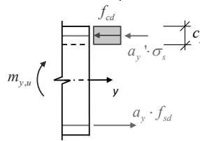
Cross-Section y-direction
