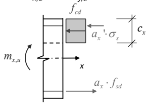
Cross-Section x-direction
