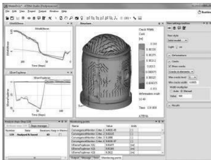
Fig 2: Over-pressure simulation of nuclear containment [Cervenka, 2020]
