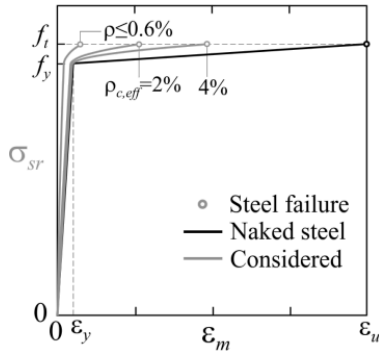
Steel EU - B500B f_t/f_u \approx 1.08 \epsilon_{su} \approx 5\%
