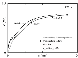
Fig. 6. Plate test IWT2 carried out by Leonhardt and Walther [15]: (a) load–deformation diagram; (b) crack pattern and principal compressive stress \sigma_3 in the main girder.
