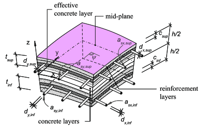
Fig. 3. Multilayer shell element – Cracked Membrane Model Usermat input parameters.
