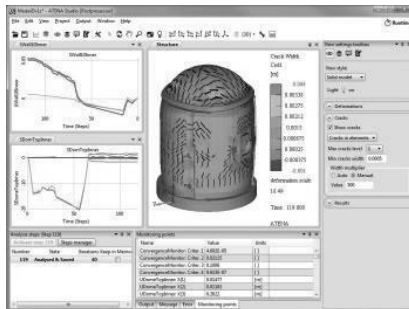
Fig 2: Over-pressure simulation of nuclear containment
