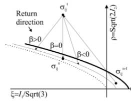
Fig. 2-22 Plastic predictor-corrector algorithm.
