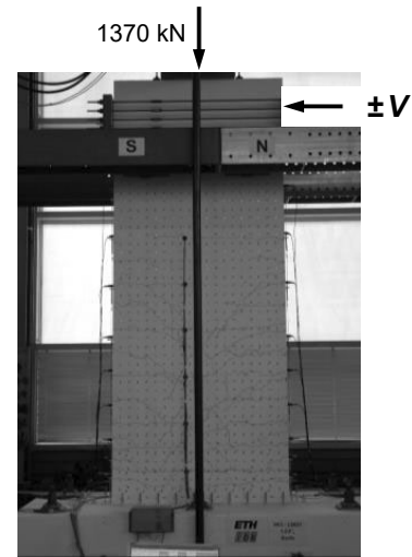
VK1: first yielding of reinforcement
