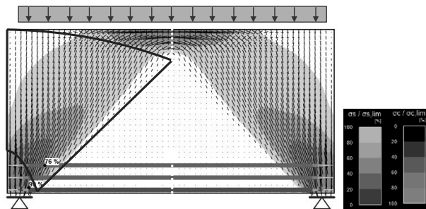
Compatible stress fields
